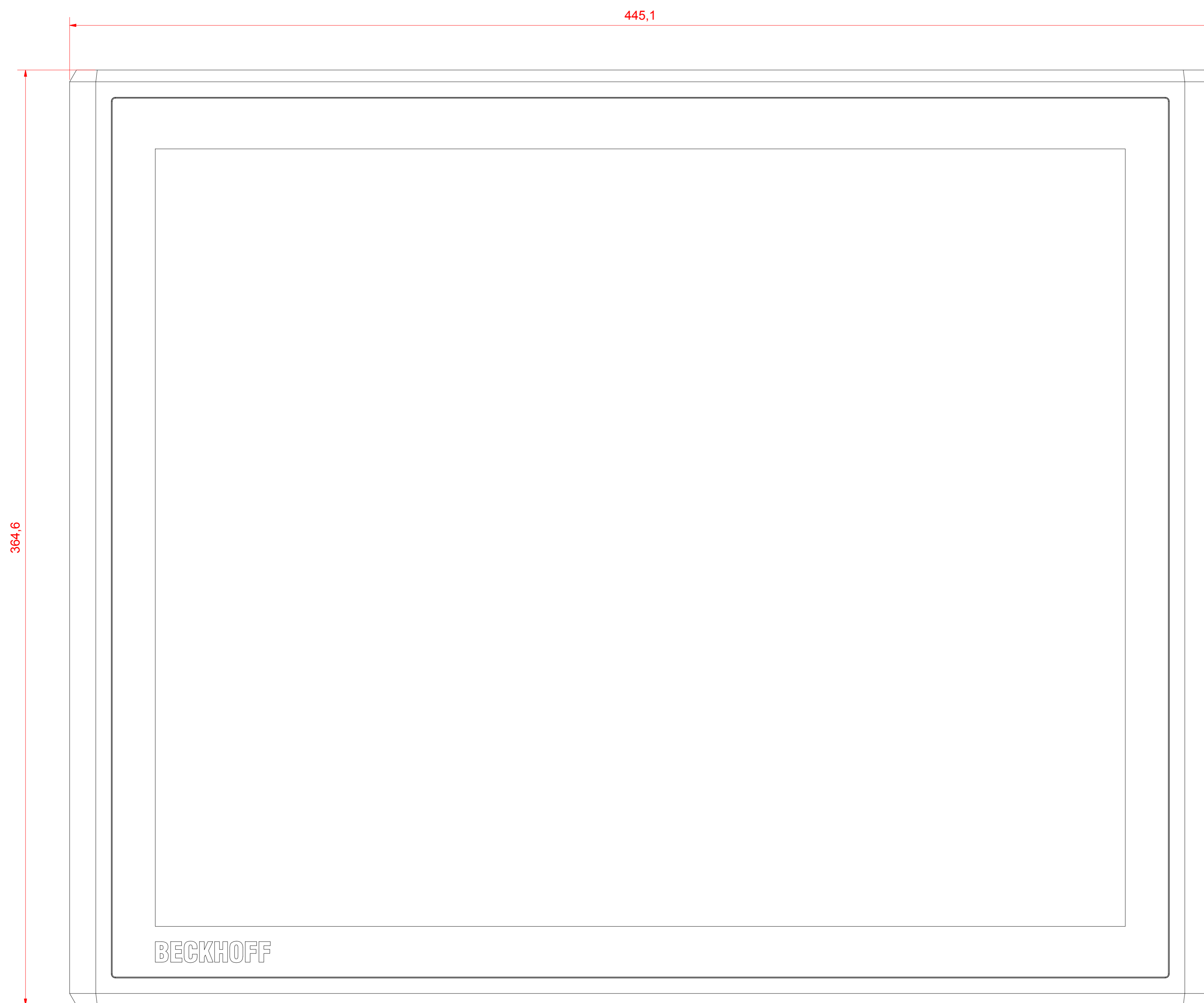
front view
