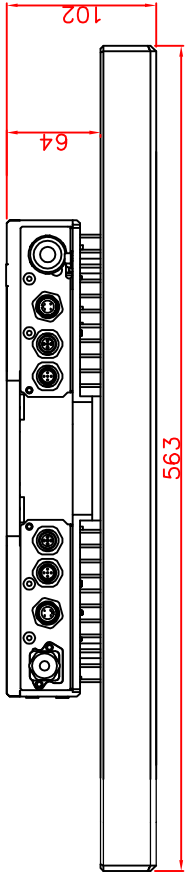
bottom view
