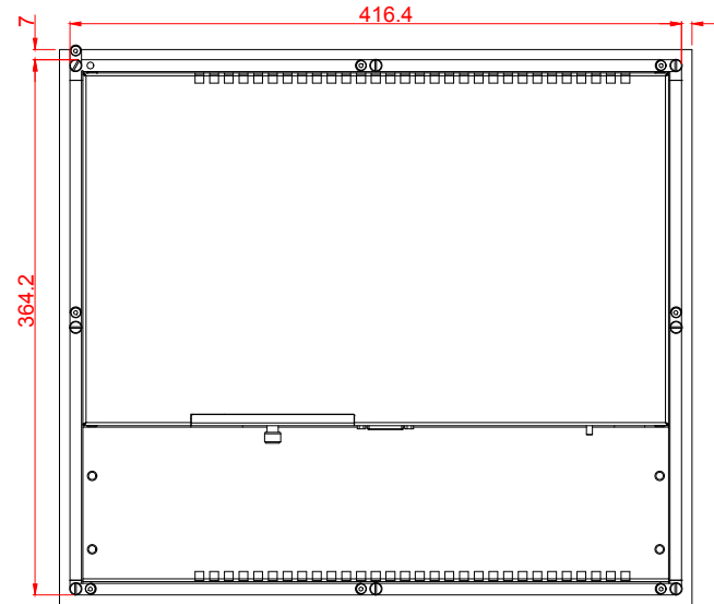
rear view
