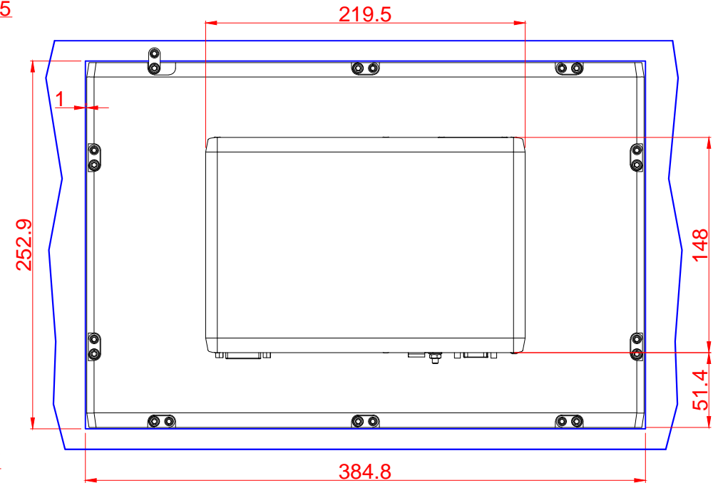
bottom view
