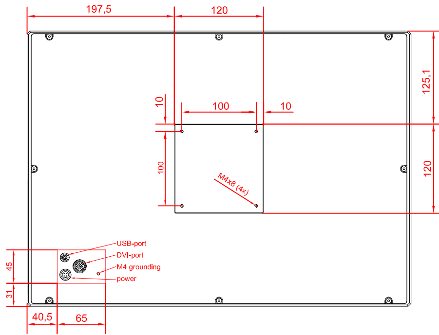
rear view
