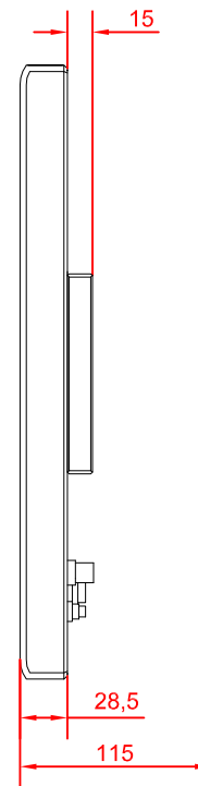
right view
