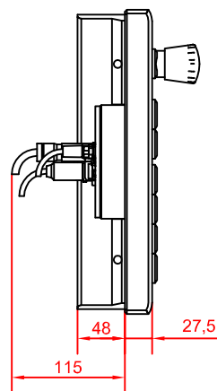
left view
