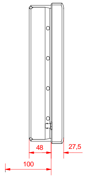
installation depth cp-link connectors left view
