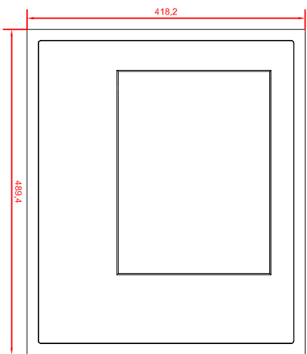
CP8632-0001 main dimensions
