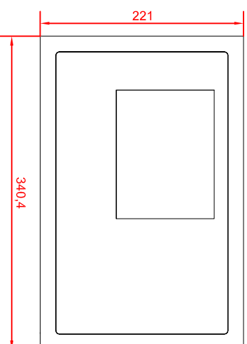
CP6929-0001 main dimensions
