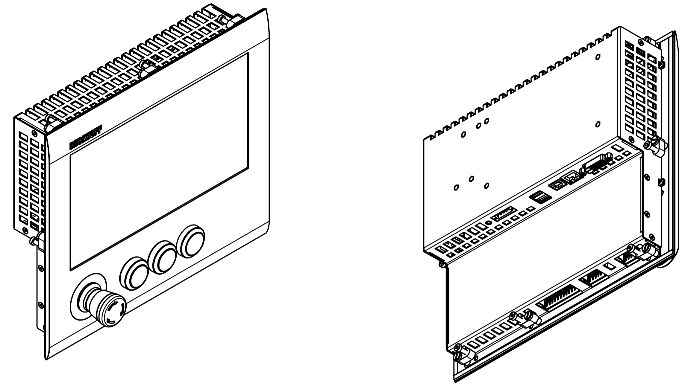
CP6900-0001 with TEW main dimensions
