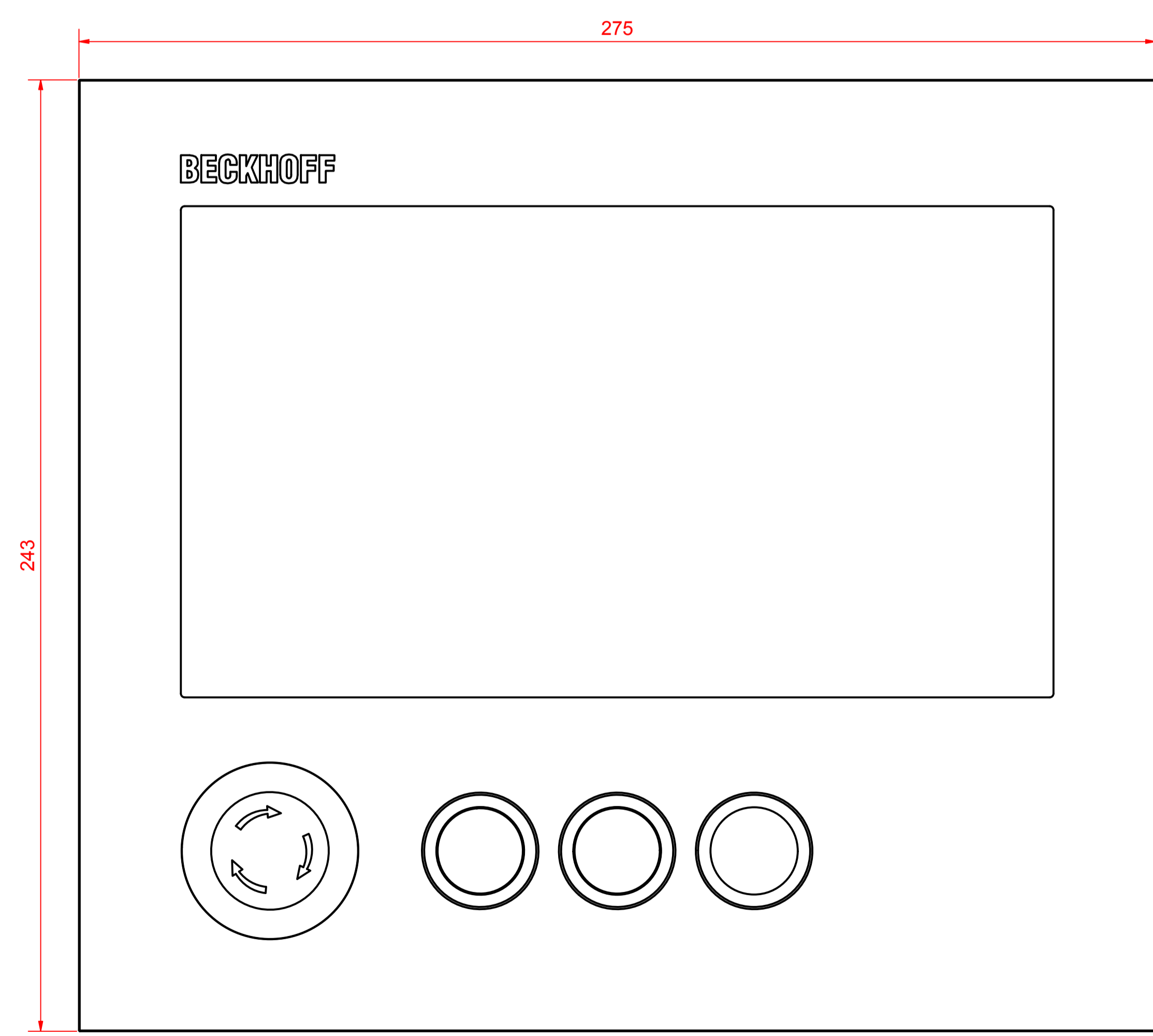
front view
