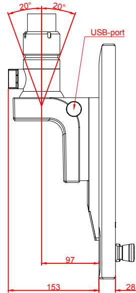
left view
