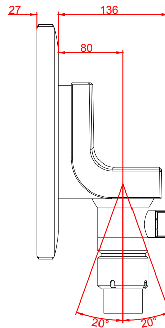
right view
