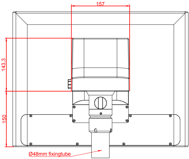
rear view
