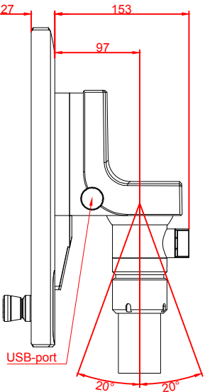
right view
