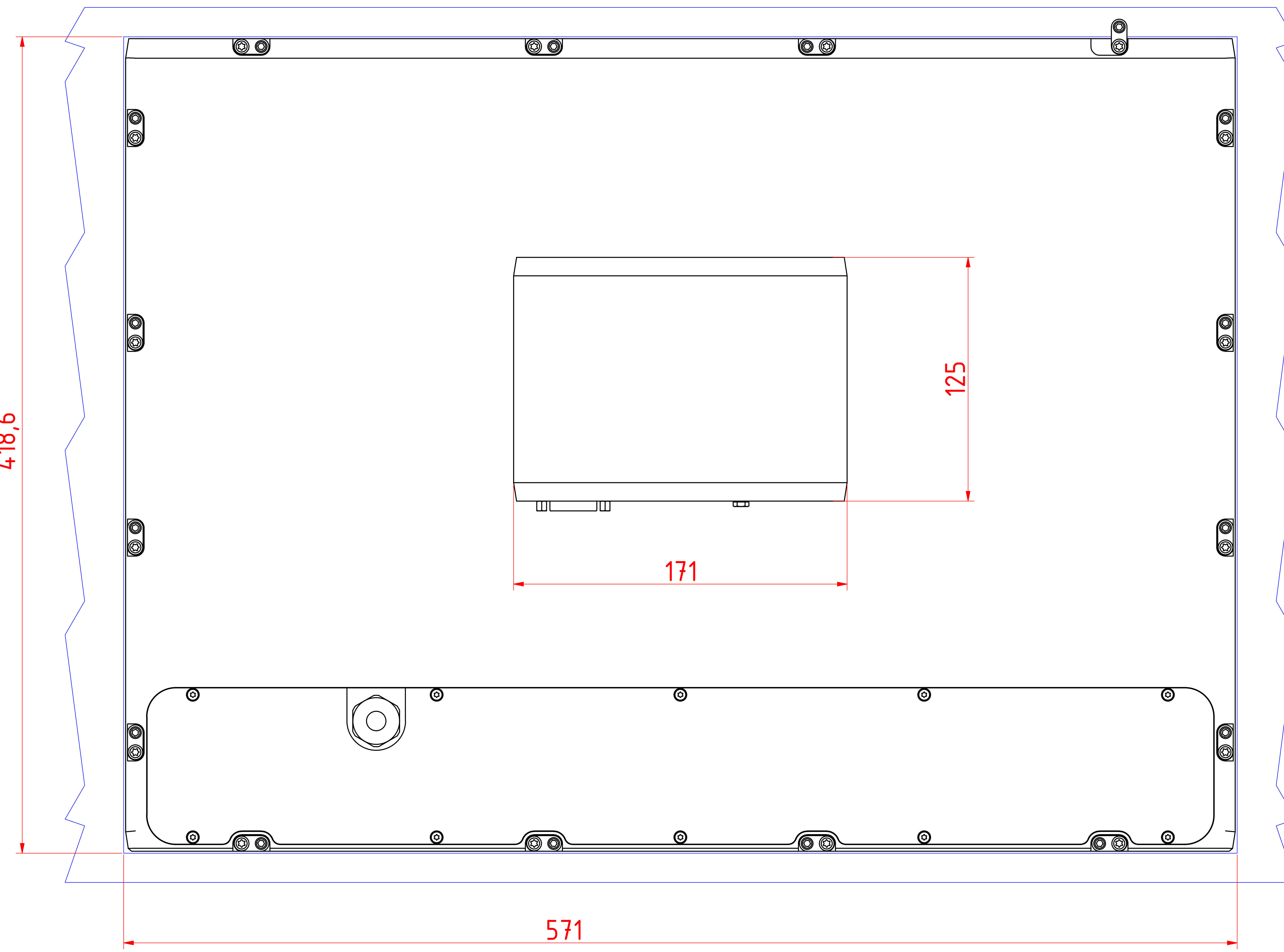
cut out dimensions: 418.6mm x 571mm rear view
