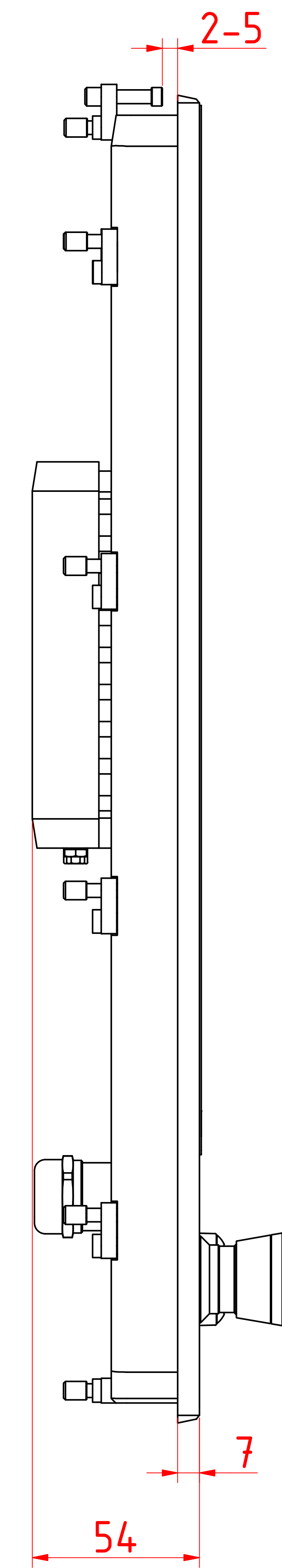
left view
