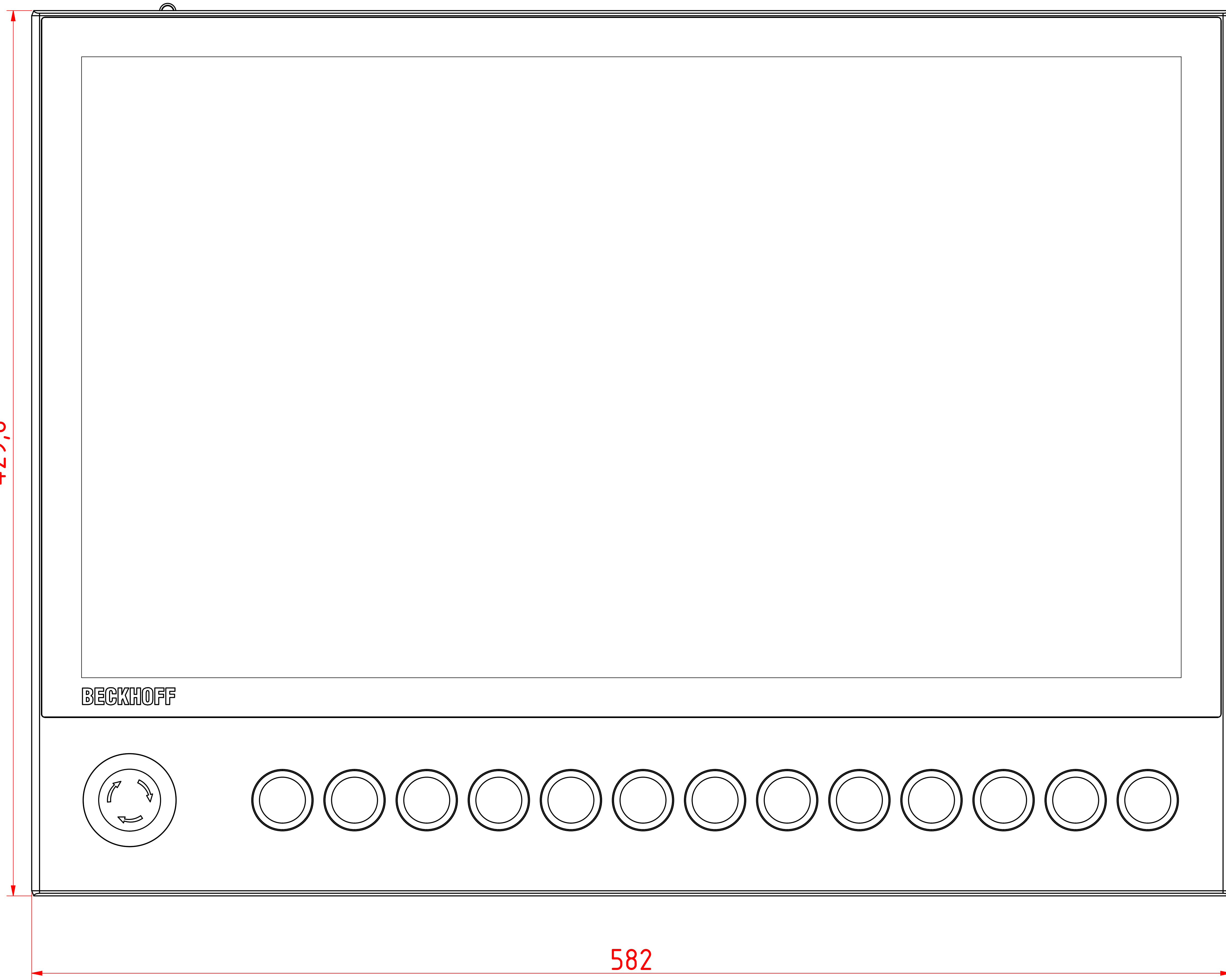
front view
