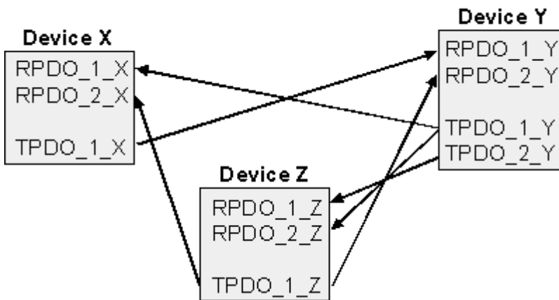
Abb. 10: PDO Linking: Peer to Peer
